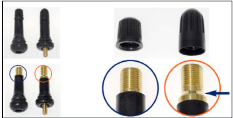
FIGURE 4B: Comparison: Valve Cap and Valve Tip Close-Up Above are the same photos comparing standard valves and TPMS valves with and without their valve caps. Note the larger tapered shoulder on the sensor valve of the TPMS.
