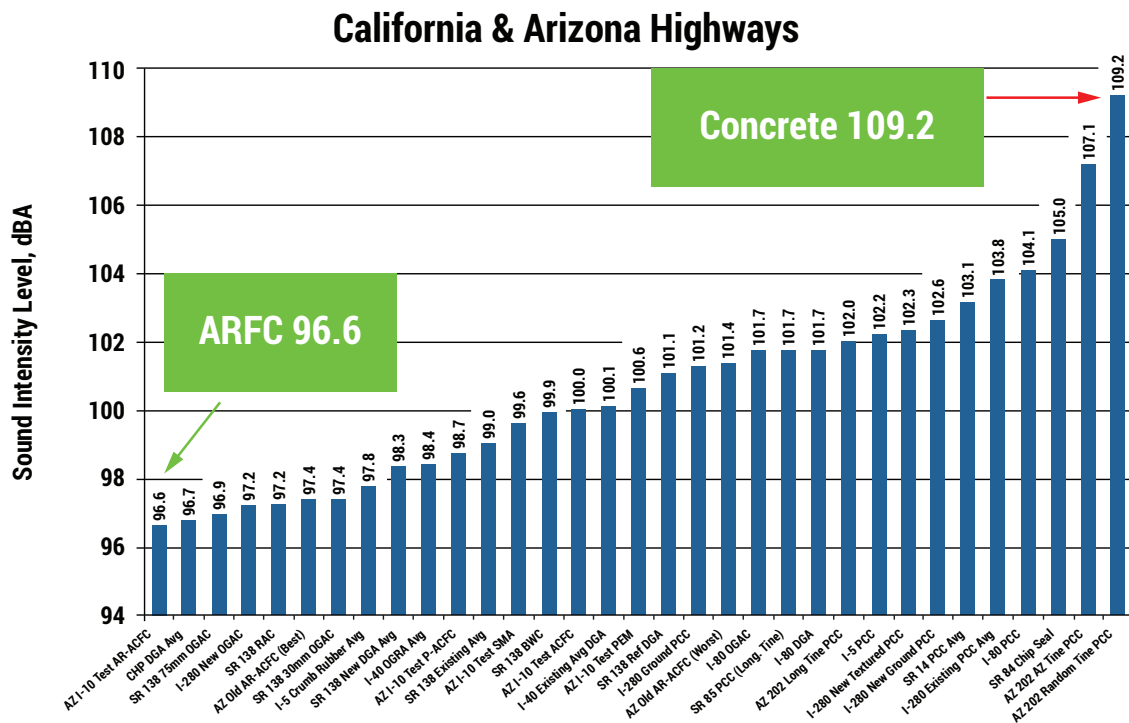
Figure 14. Noise data from highways in Arizona and California (from (G. Way, 2012))
