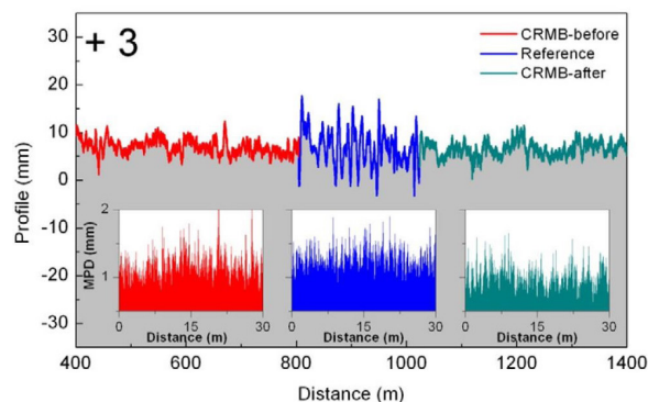
Figure 16. Showing the effect of rubber in producing smoother pavements (from (Vázquez et al., 2016))
